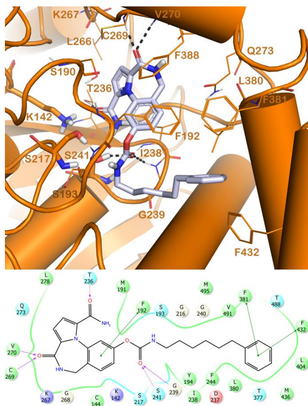
Figure 5. Binding modes of 3m (light gray sticks) into h/r FAAH enzyme (orange cartoon, PDB ID: 3PPM) binding site. The residues forming the catalytic triad (K142, S217 and S241) are reported as sticks while the other residues of the binding site are reported as lines. The non-polar hydrogens were removed for clarity. The picture was generated by means of PyMOL.
