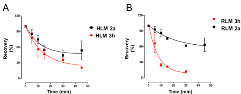
Figure 7. CYP-dependent metabolic depletion of 5 \mu\text{M} 3h and 2a in human (HLM, panel A) and rat liver (RLM, panel B) microsomal preparations. Results are presented graphically as percentage of compound recovery (100% at time 0 min) as a function of incubation time. Data are presented as mean \pm SEM, of three different experiments.
